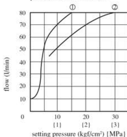
① MR*-03-A-10T 32 cSt [32mm²/s] ② MR*-03-B-10T pressure-flow characteristic
