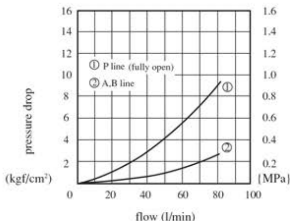
MR*-03-*-10T pressure drop characteristic
